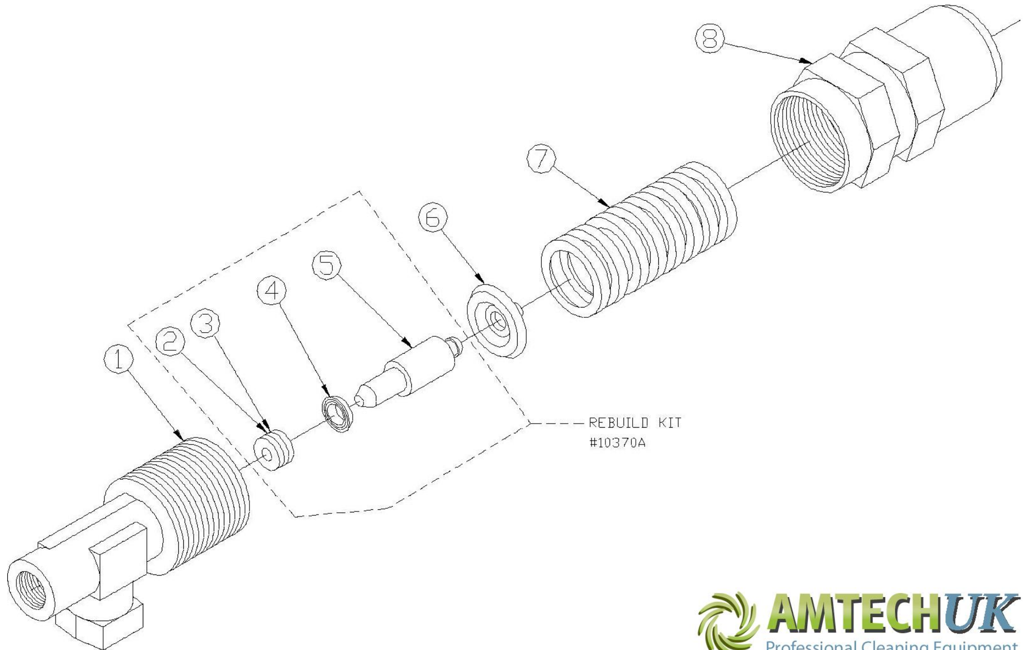
#10370A Pressure Regulator Rebuild Kit Assembly Diagram.
